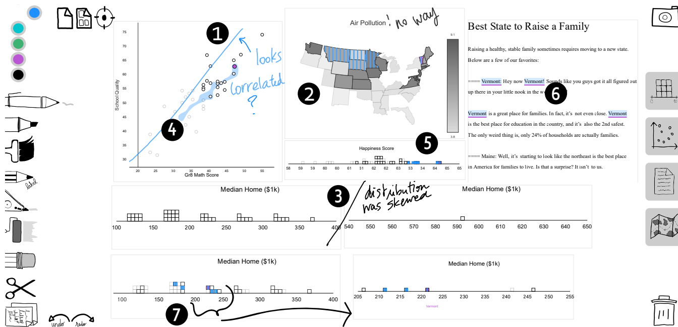
Figure 4: Depiction of the canvas of a data journalist organizing their workspace and annotating findings (1-ink \downarrow , 2-cut \circ , 3-remove \ominus ) and interacting on the data to identify salient subsets (4-hide \square , 5-highlight \color{blue} , 6-paint \color{blue} and label \textcircled{6} , and 7-copy \square a subset of a histogram).
